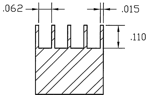
STANDARD DETAIL .110 DP BLADE TEETH
